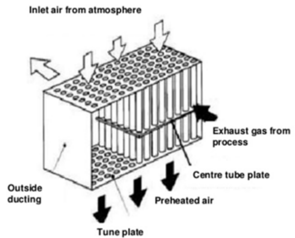
Figure 19: Metallic recuperator
