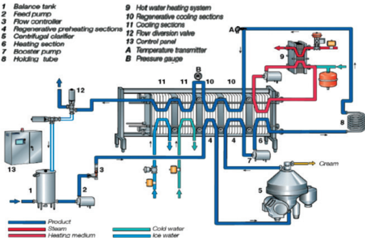
Figure 46: Pasteurization process
