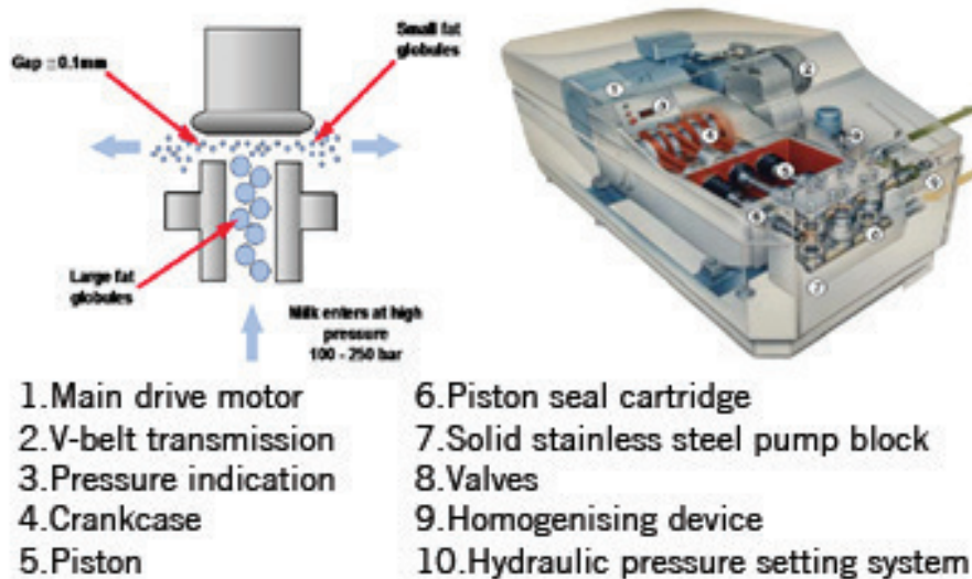
Figure 10: Homogenization Process
