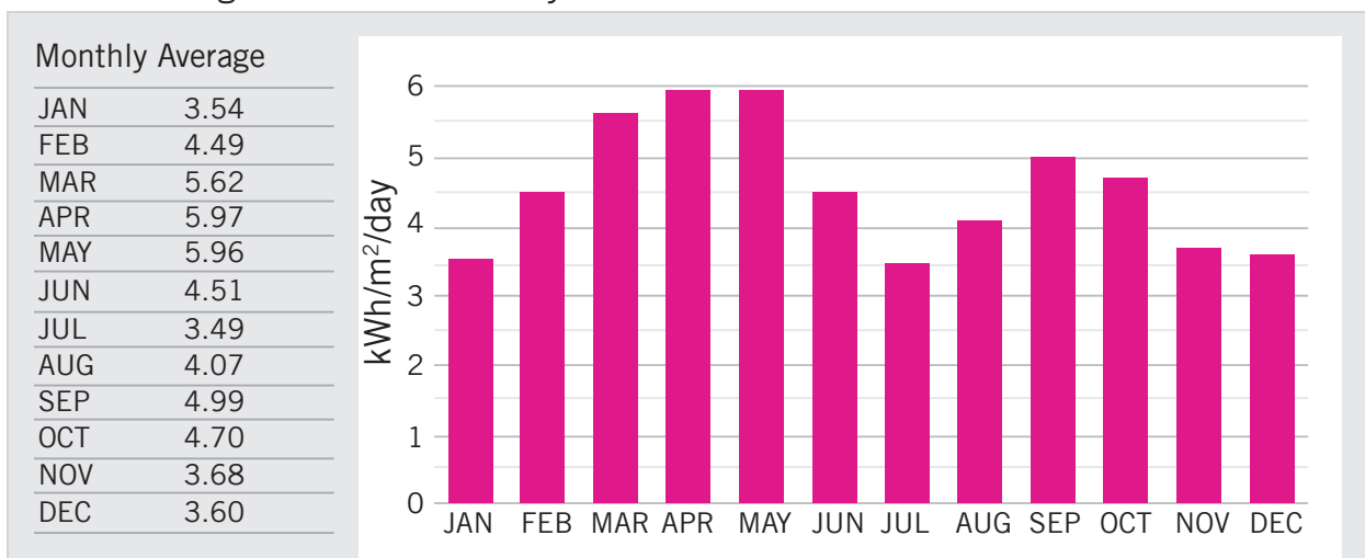
Figure 47: Solar Irradiance
