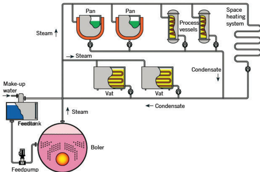
Figure 17: Typical condensate recovery system
