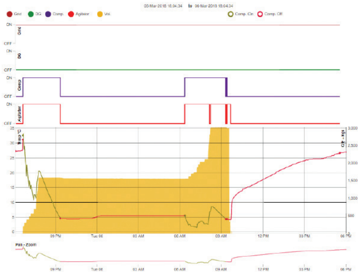
Figure 37: Chilling graph
