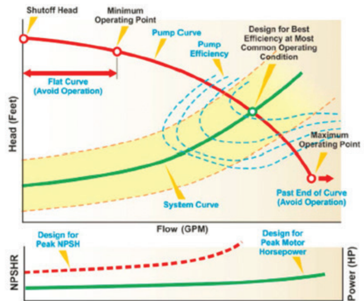
Figure 41: Pump Characteristic Curve
