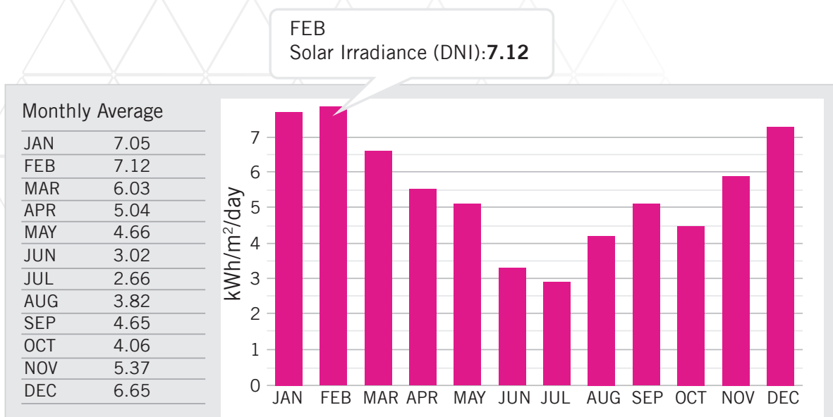
Figure 48: Solar Irradiance
