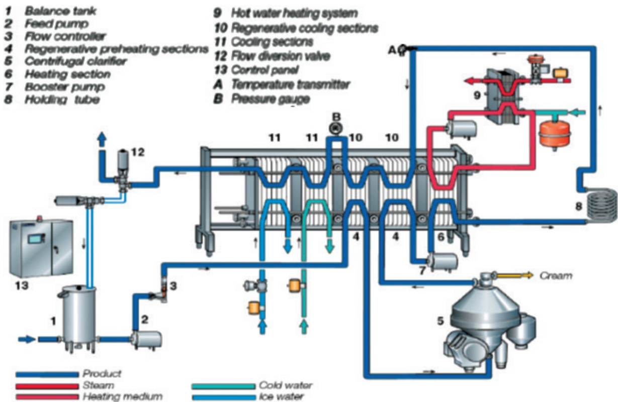
Figure 47: Pasteurization process
