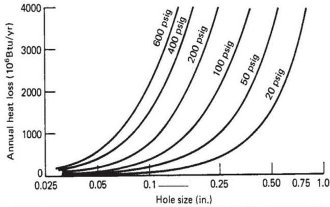
Figure 20: Steam Loss Chart
