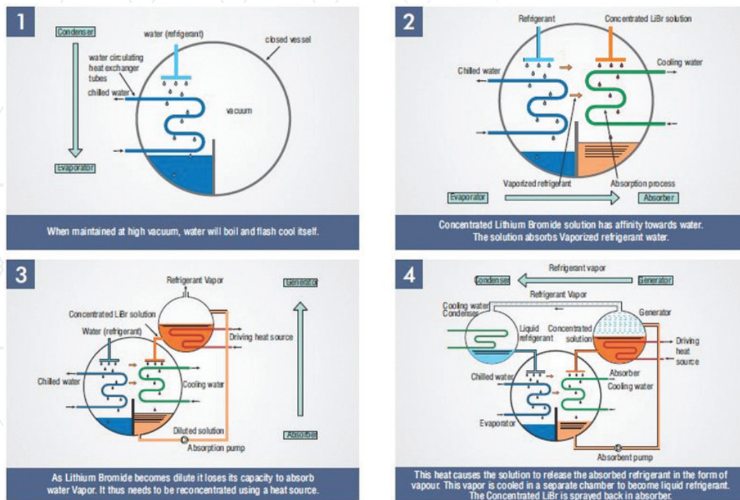
Figure 28: VAM working
