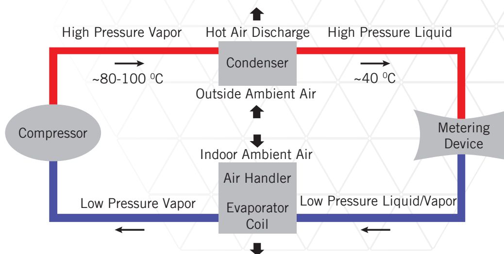
Figure 29: Vapour Compression Cycle
