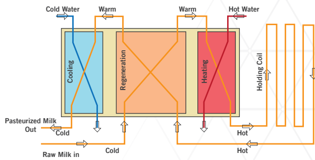
Figure 9: Pasteurization process
