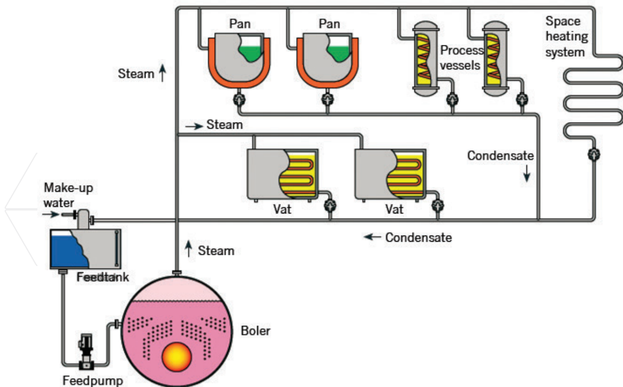
Figure 18: Typical condensate recovery system
