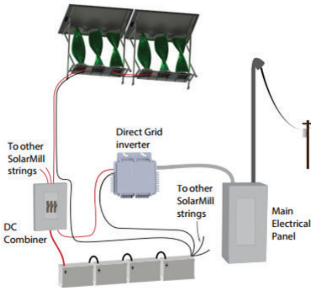
Figure 52 Hybrid mill connected to supply
