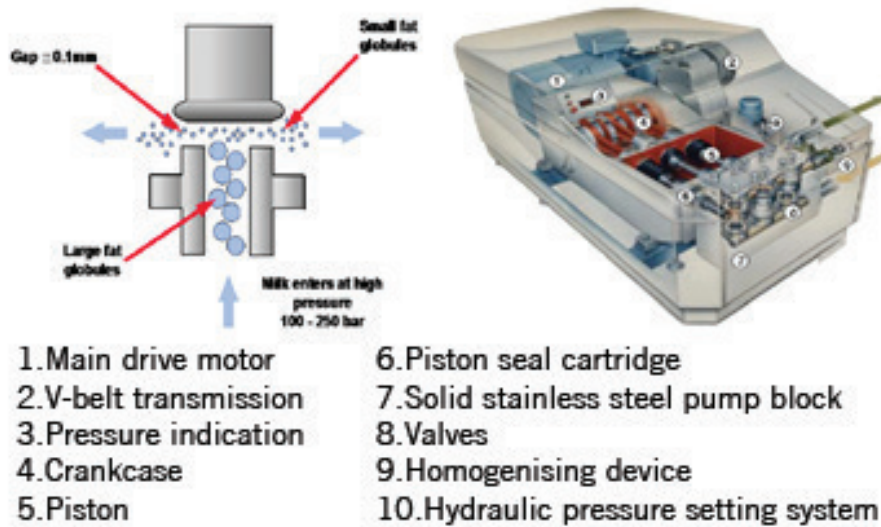
Figure 11: Homogenization Process
