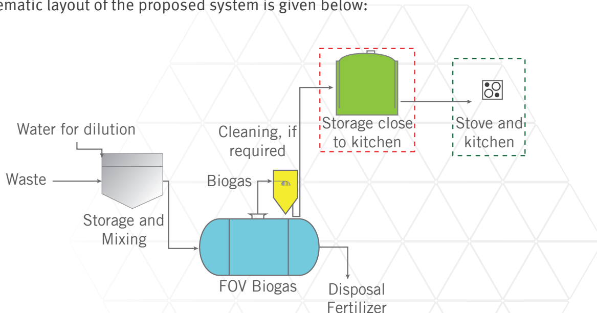
Figure 44: Layout of FOV Biogas Technology
